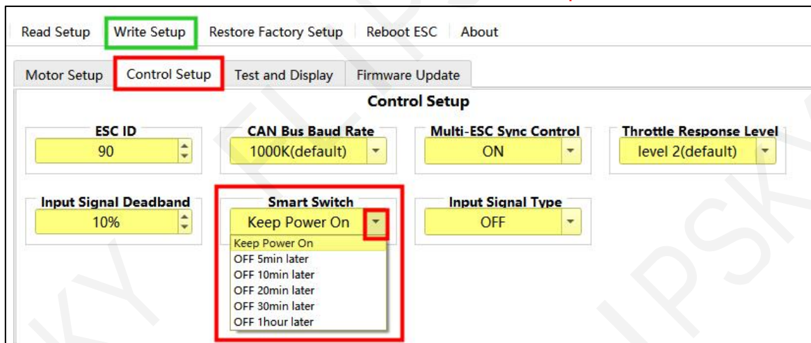
Screenshot 7-7 Smart Switch Setup
