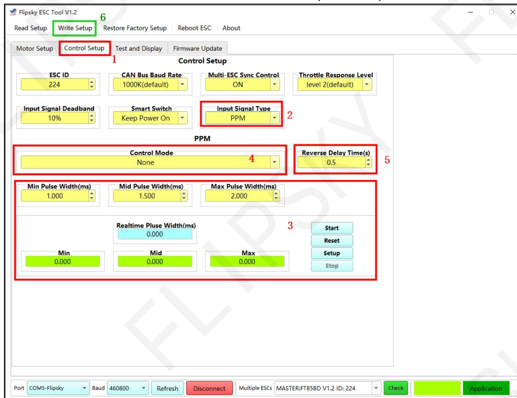
Screenshot 7-16 PPM Input Setup
