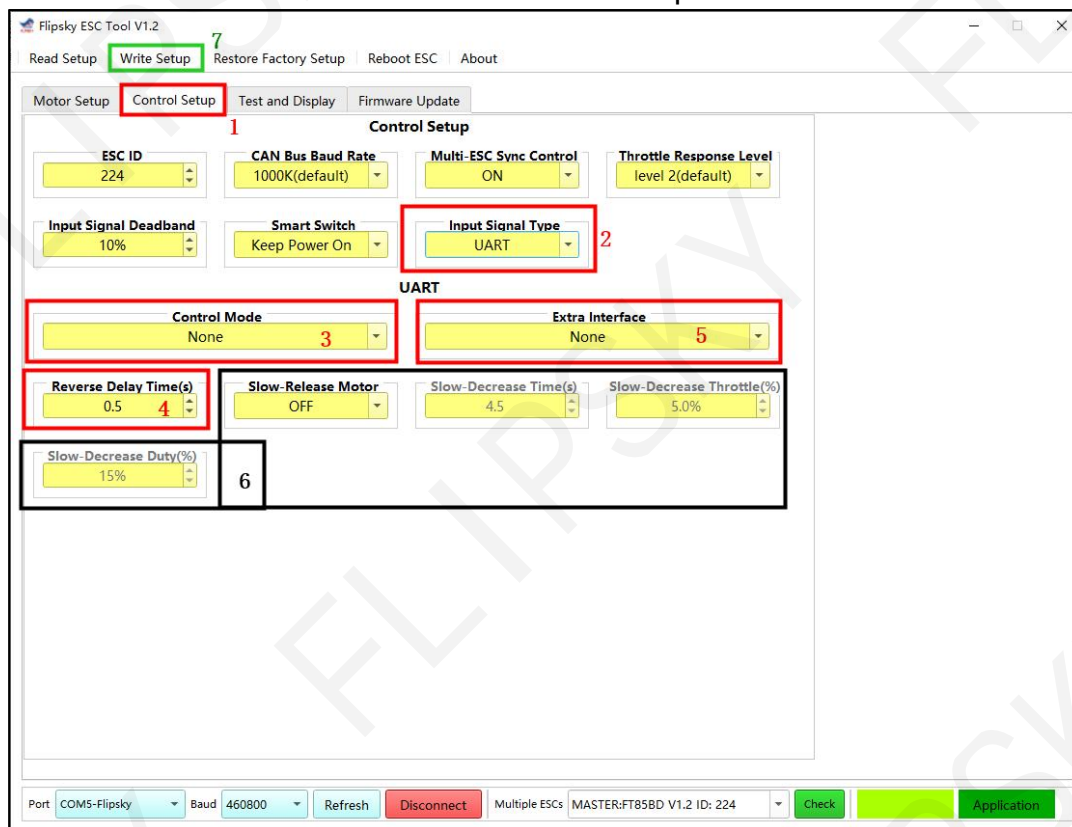
Screenshot 7-11 UART Setup Interface
