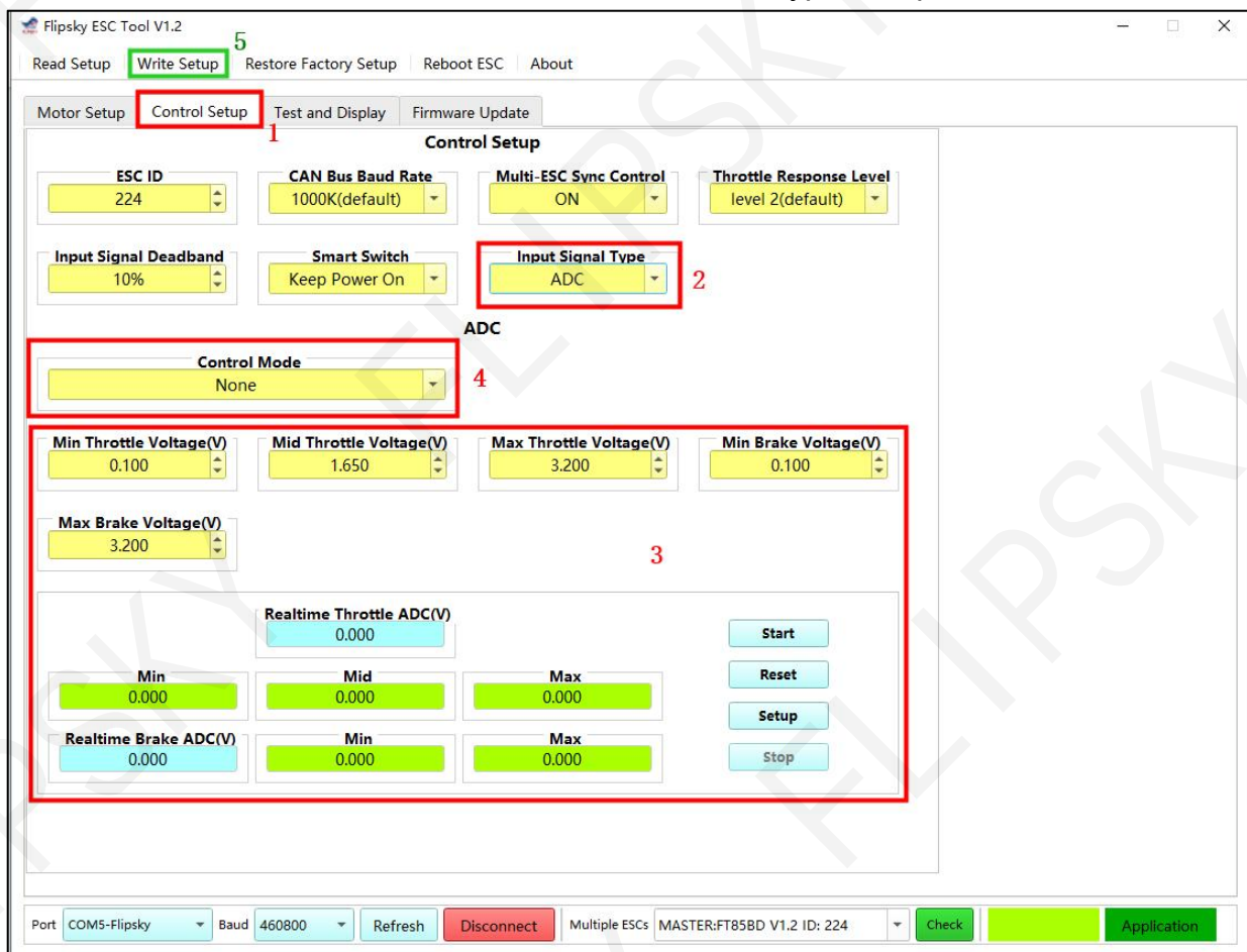
Screenshot 7-26. ADC Control Type Setup
